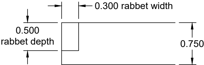
RABBET DETAIL
